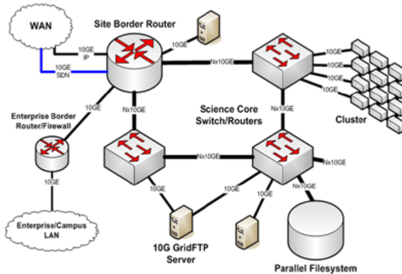
A Typical Network Lay Out for a Complex High End Compute Intensive Server Installation
